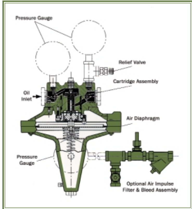
View of the MRO ratio regulator showing its internal components and the oil flow path.
