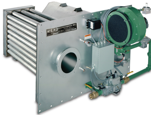
RHT Indirect Air Heater (recirculating high temperature indirect air heater)
