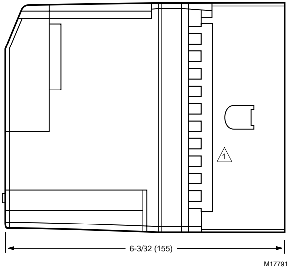
Fig. 2. Mounting dimensions of EC7895; RM7895; RM7896 Relay Module, Q7800A Subbase and Q7800B Subbase, respectively, in in. (mm).
