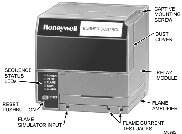
Fig. 1. Relay Module and sequence status LEDs.
